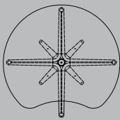
A (Apple) WK-TP-A85-25 8650W/ 754D/ 25THK mm WK-TP-A100-25 1000W/ 899D/ 25THK mm
