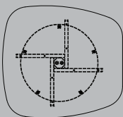
B (Tracut) WK-TP-B85-25 850W/ 795D/ 25THK mm WK-TP-B100-25 1000W/ 892D/ 25THK mm
