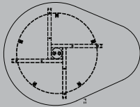
F (Pear) WK-TP-F85-25 1000W/ 850D/ 25THK mm
