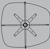
B (Tracute) WK-TP-B70-25 700W/ 649D/ 25THK mm WK-TP-B85-25 850W/ 795D/ 25THK mm
